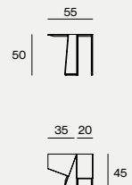
DIMENSIONS 55X45X50H
