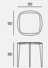
DIMENSIONS 50X50X50H
