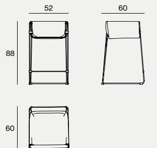
DIMENSIONS 55X60X88H
