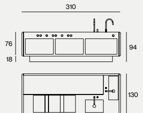
DIMENSIONS 310X130X94H
