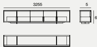
DIMENSIONS 325X55X65H
