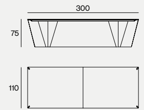
DIMENSIONS 300X110X75H
