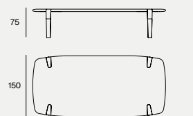
DIMENSIONS 330X150X75H
