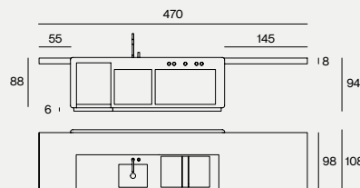
DIMENSIONS 470X108X94H
