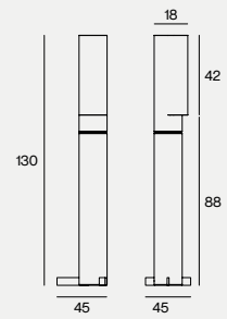
DIMENSIONS 45X45X130H
