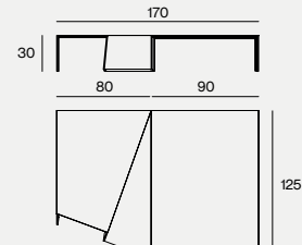
DIMENSIONS 170X125X30H
