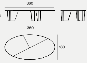
DIMENSIONS 360X180X75H
