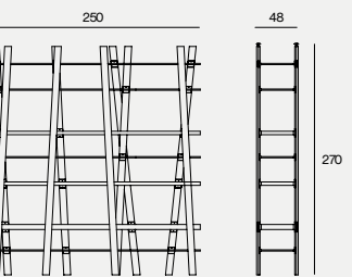
DIMENSIONS 250X48X270H
