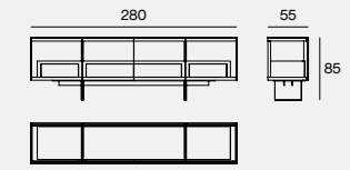
DIMENSIONS 280X55X85H
