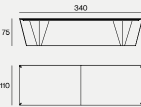
DIMENSIONS 340X110X75H
