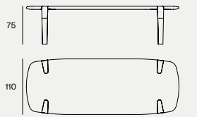
DIMENSIONS 300X110X75H
